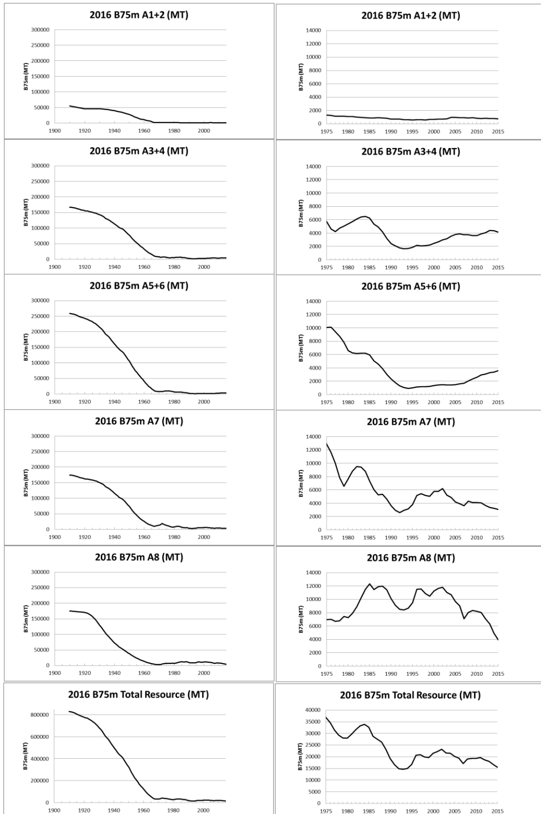
Figure 2: Trajectories of male B75m (MT) estimated from recent assessments for each super-area and for the resource as a whole. The left panel shows trajectories from 1910, whilst the right panel shows only the 1975+ period.
