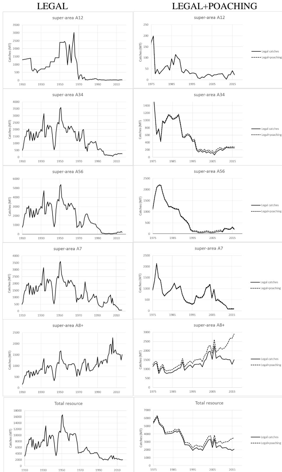
Figure 3: Trajectories of the catches (legal) for each super-area and the resource as a whole. Note different y-axis scales. The left panel shows Legal catches from 1910 onwards, whilst the right panel compares the Legal with the Legal+poaching estimates for 1975 onwards.
